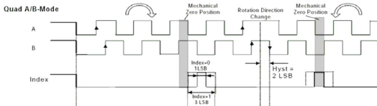
Output Waves
