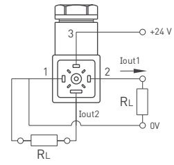
0-20mA and 4-20mA Output
